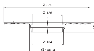
Kingspan ESSMANN renovation gully washer for old gullies, inlet inside diameter 150-250 mm
